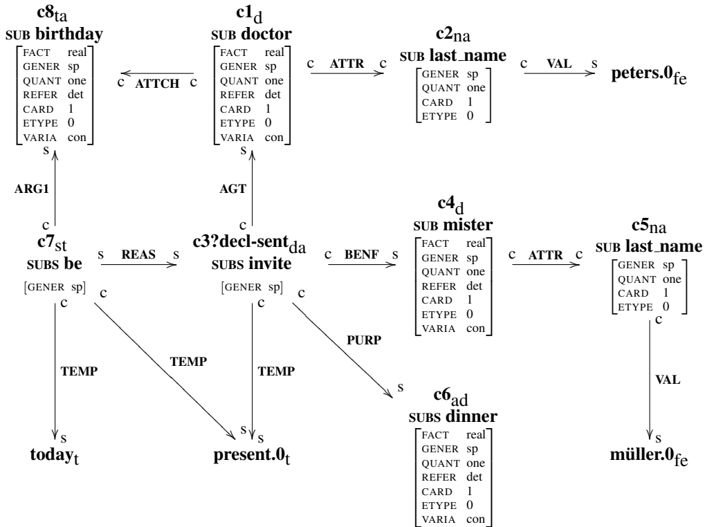
Figure 1: Example of an SN from the WOCADI parser (node names are translated from German). The sort of a node is written as a subscript of the node name. The feature structure below a node name shows layer features and their values. Each arc is labeled with a MultiNet relation. To simplify the graph topology, SUB and SUBS arcs are folded below the start nodes. Labels at the start and at the end of an arc indicate the so-called knowledge type, e.g. categorical (c) and situational (s); see for details.
