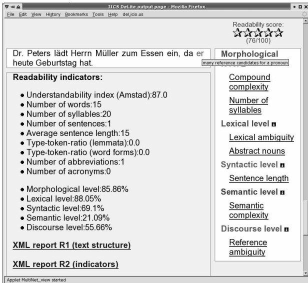
Figure 2: Screenshot of DeLite's GUI.
